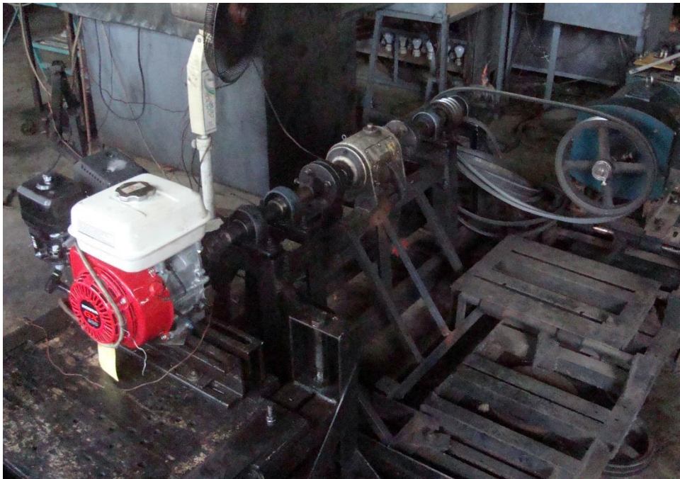
Figure 2. Test set-up of the HONDA GX200H QTP Gasoline Engine
