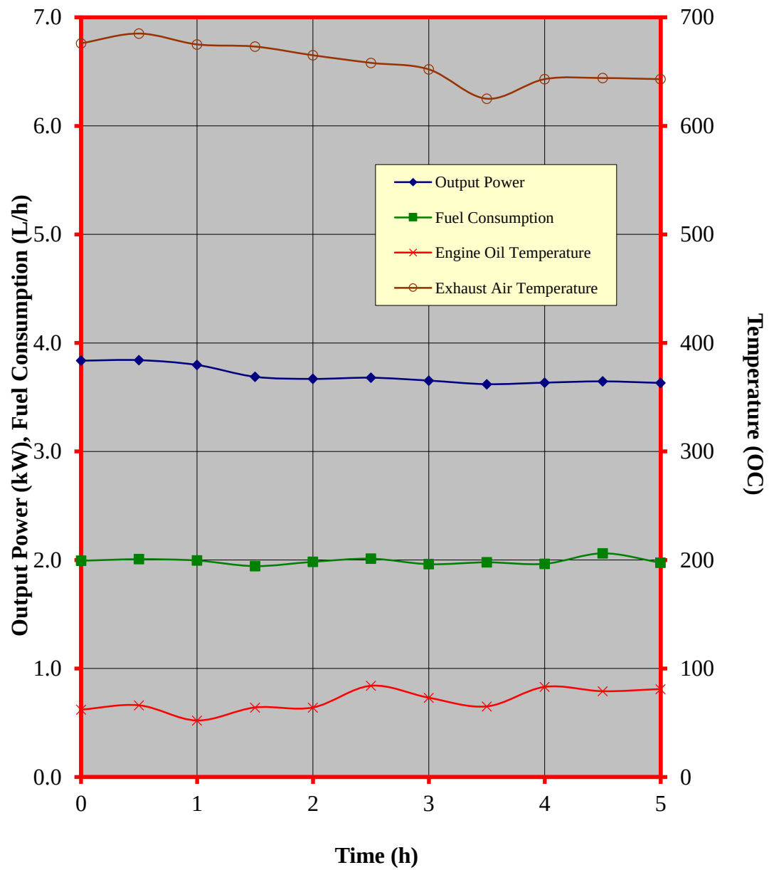
Figure 4. Performance characteristic curves during the continuous running test of the HONDA GX200H QTP gasoline engine
