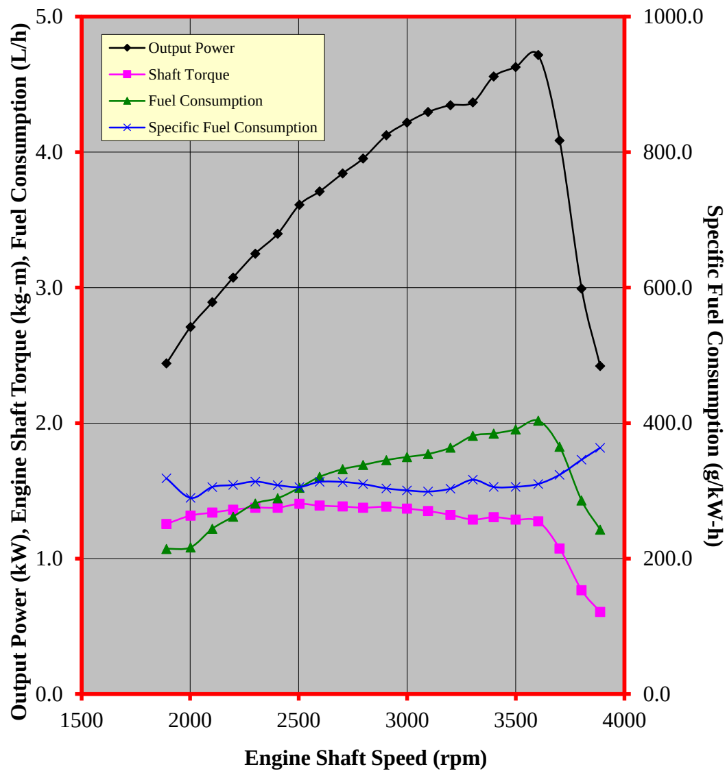
Figure 3. Performance characteristic curves of the HONDA GX200H QTP gasoline engine
